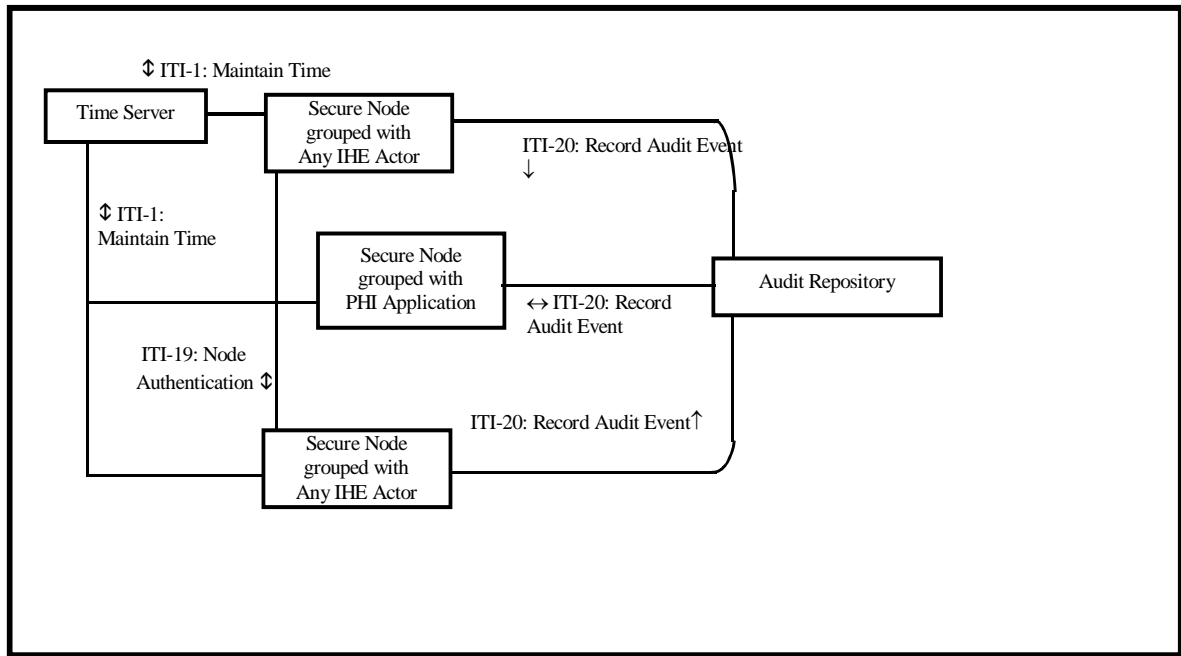
1485 Figure 9.4-1. Audit Trail and Node Authentication Diagram
