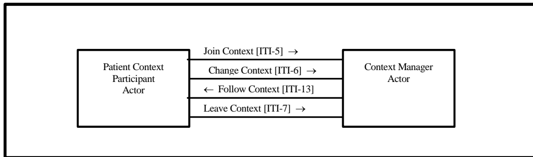
1080 Figure 6.1-1 Patient Synchronized Applications Profile Actor Diagram
